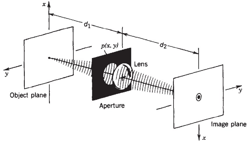
Figure 10.3-4 A single-lens imaging system.
