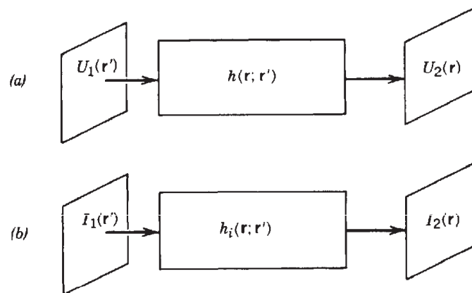
Figure 10.3-3 (a) The complex amplitudes of light at the input and output planes of an optical system illuminated by coherent light are related by a linear system with impulse-response function h(\mathbf{r}; \mathbf{r}') . (b) The intensities of light at the input and output planes of an optical system illuminated by incoherent light are related by a linear system with impulse-response function h_i(\mathbf{r}; \mathbf{r}') = \sigma |h(\mathbf{r}; \mathbf{r}')|^2 .
