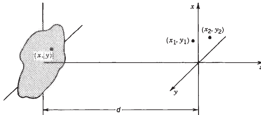
Figure 10.3-7 Radiation from an incoherent source in free space.
