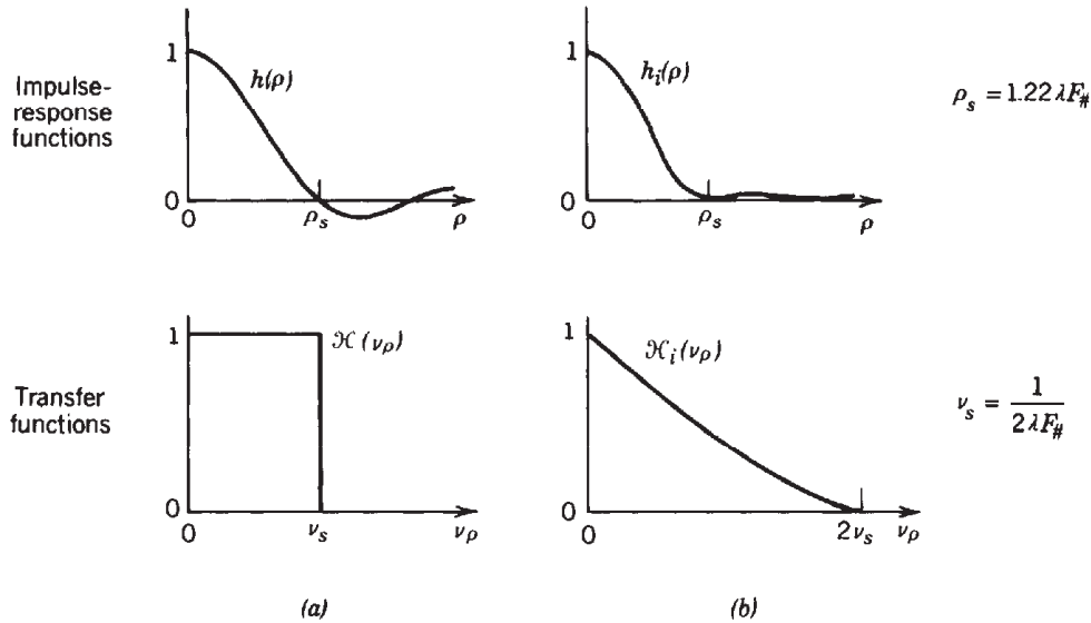
Figure 10.3-5 Impulse-response functions and transfer functions of a single-lens focused diffraction-limited imaging system with a circular aperture and F -number F_{\#} under (a) coherent and (b) incoherent illumination.
